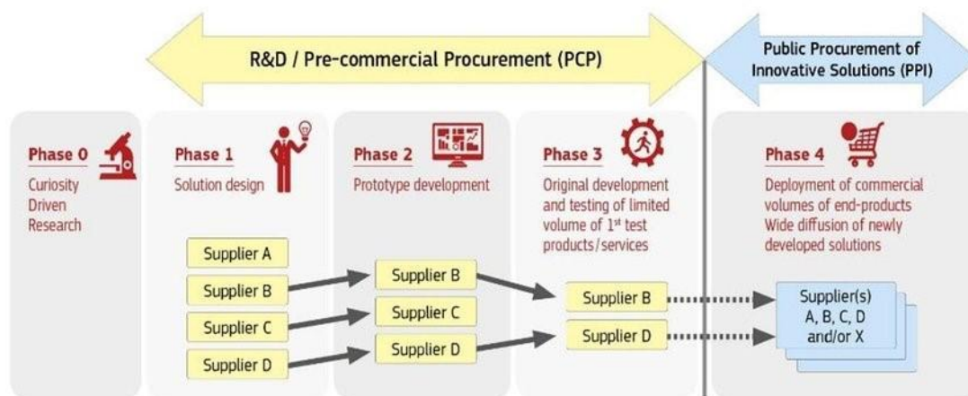
Figure 2 PCP and PPI, according to the European Commission (2016). Based on "Pre-commercial procurement: driving innovation to ensure sustainable high quality public services in Europe", COM(2007) 799 final.
